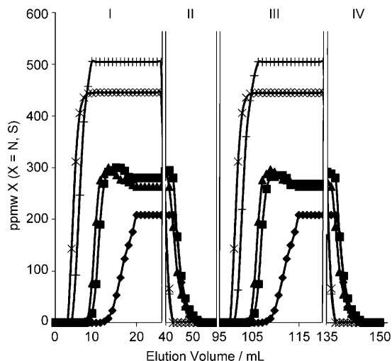
Figure 4. Breakthrough experiment at 298 K on a MIL-100(Fe) column at 298 K with a solution of 0.011 M indole ( \blacklozenge ), 0.011 M 1,2-dimethylcarbazole ( \blacksquare ), 0.014 M N-methylcarbazole ( \blacktriangle ), 0.009 M benzothio-phenone ( \times ), and 0.009 M dibenzothiophene ( + ) dissolved in H/T (a total of 950 ppmw S and 750 ppmw N). All curves are corrected for the dead volume. Sections I and III: adsorption of the mixtures; sections II and IV: the final part of the regeneration in pure toluene. Between adsorption and desorption, the column was flushed with pure toluene (13.5 mL; 10 mL of which is dead volume); between desorption and adsorption, the column is flushed with pure H/T to be regenerated (40 mL; not shown).
